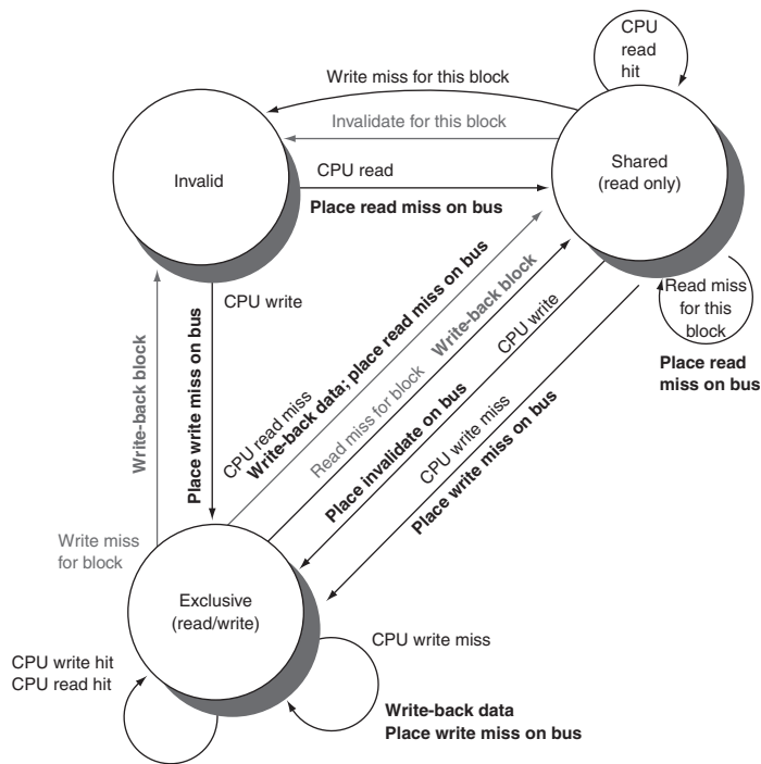
e5.12.10, the activities on a transition are shown in bold.
