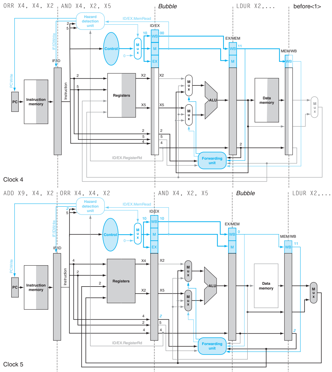
FIGURE e4.13.19 Clock cycles 4 and 5 of the instruction sequence on page 366.e26 with a load replacing SUB . The bubble is inserted in the pipeline in clock cycle 4, and then the and instruction is allowed to proceed in clock cycle 5. The forwarding unit is highlighted in clock cycle 5 because it is forwarding data from LDUR to the ALU. Note that in clock cycle 4, the forwarding unit forwards the address of the LDUR as if it were the contents of register X2 ; this is rendered harmless by the insertion of the bubble. The bold lines are those active in a clock cycle, and the italicized register numbers in color indicate a hazard.
